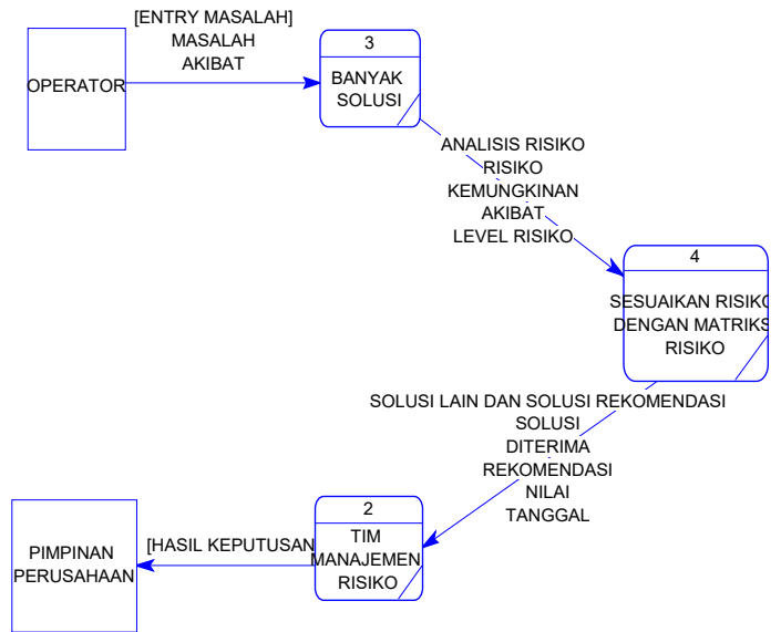
Gambar 5 Data Flow Diagram Level 1
